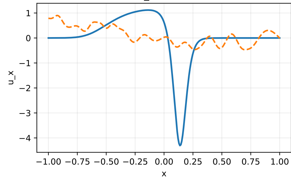
u_x at t=0
