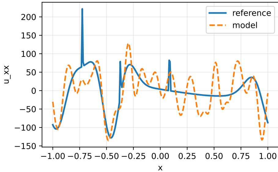
u_{xx} at t=0.5
