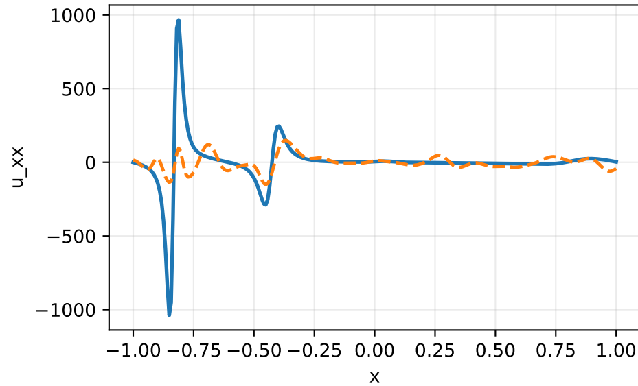
u_{xx} at t=1
