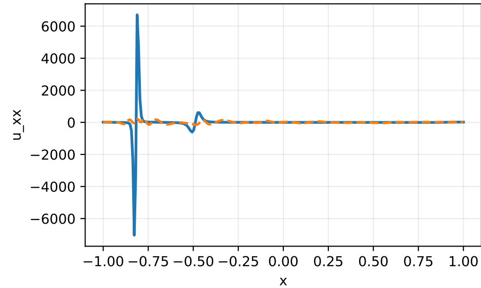
u_{xx} at t=-0.004
