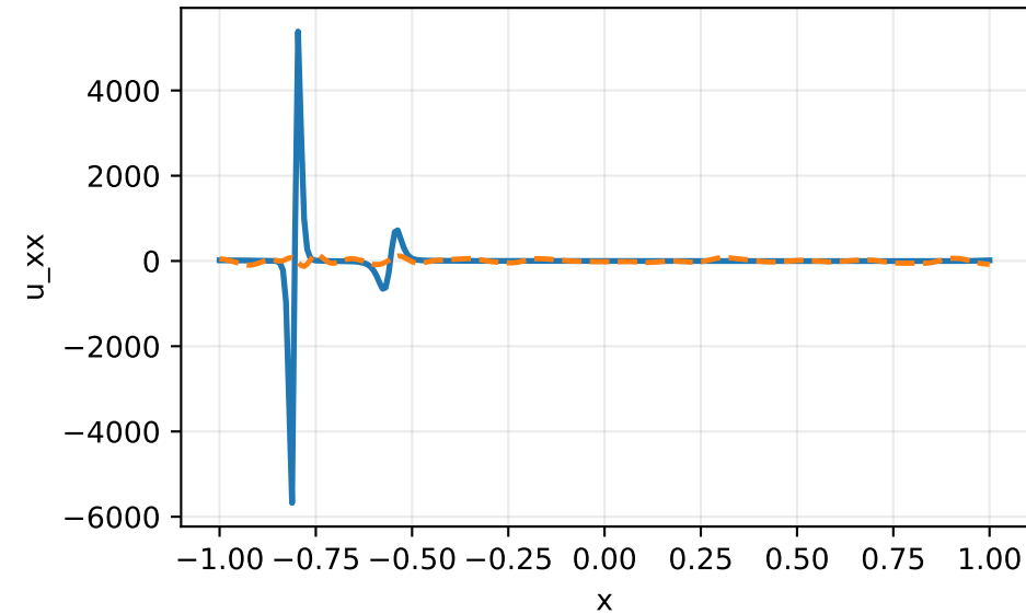
u_{xx} at t=0.5
