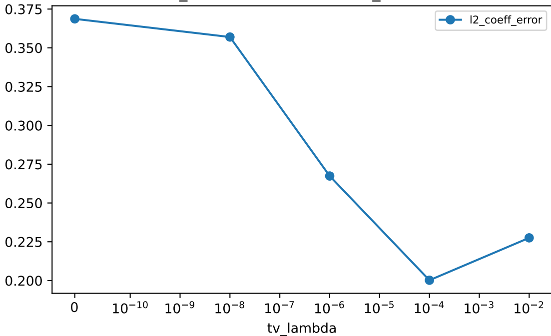
tv_u: PDE coeff error vs tv_lambda
