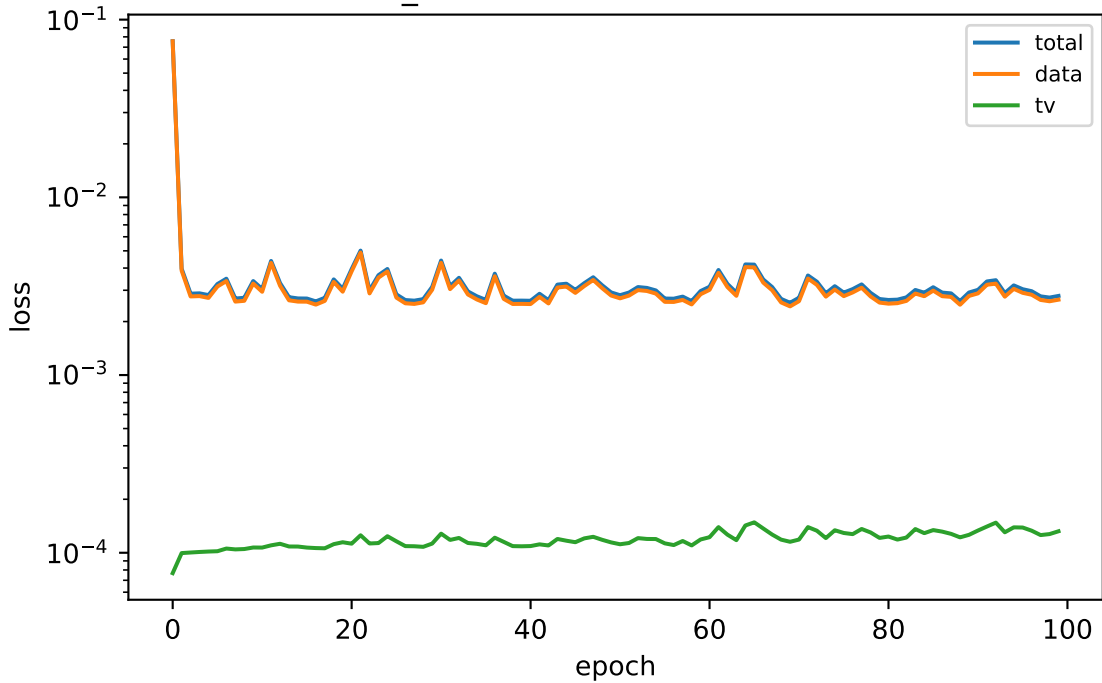
tv_ux lambda=1e-06 seed=0
