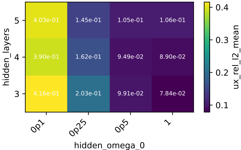
Mean ux relative L2 error
