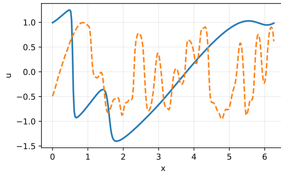
u at t=0.498
