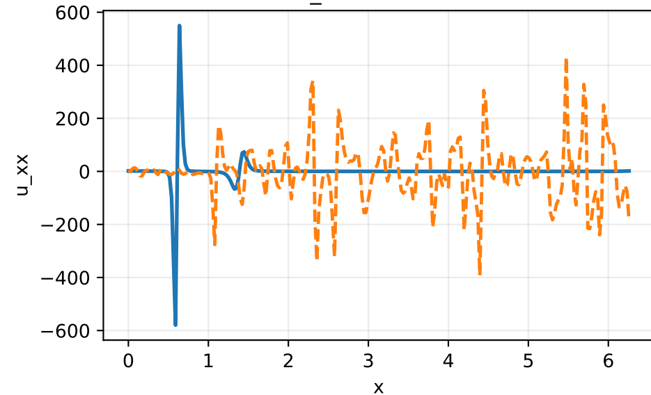
u_xx at t=0.75
