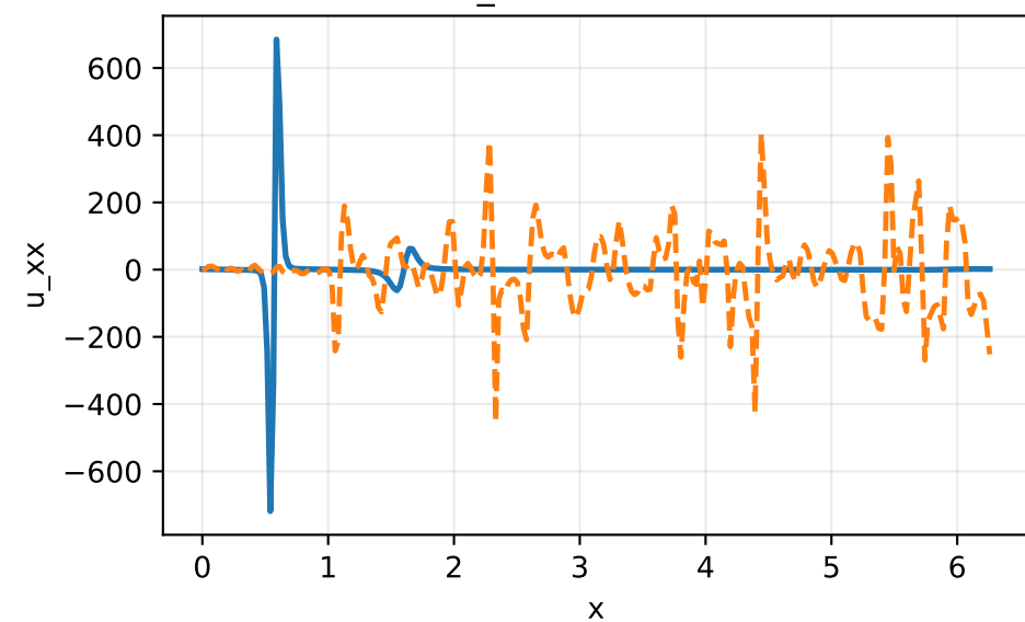
u_xx at t=0.498
