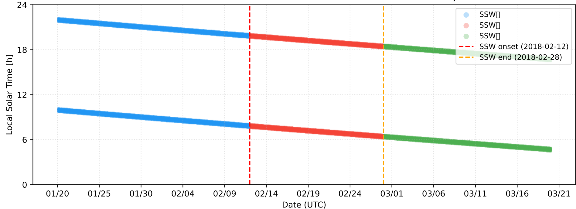
2018 NH SSW Swarm-A — Date vs Local Solar Time N=113,171
