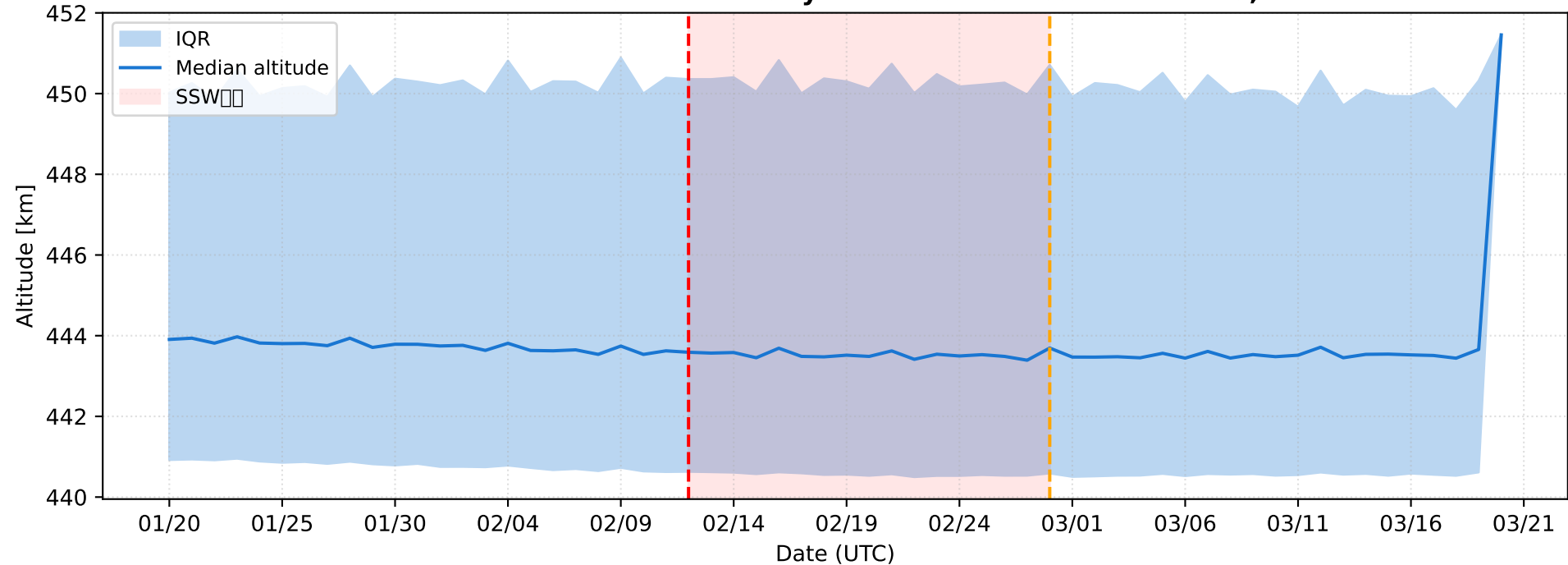
2018 NH SSW Swarm-A — Daily Altitude Distribution N=113,171
