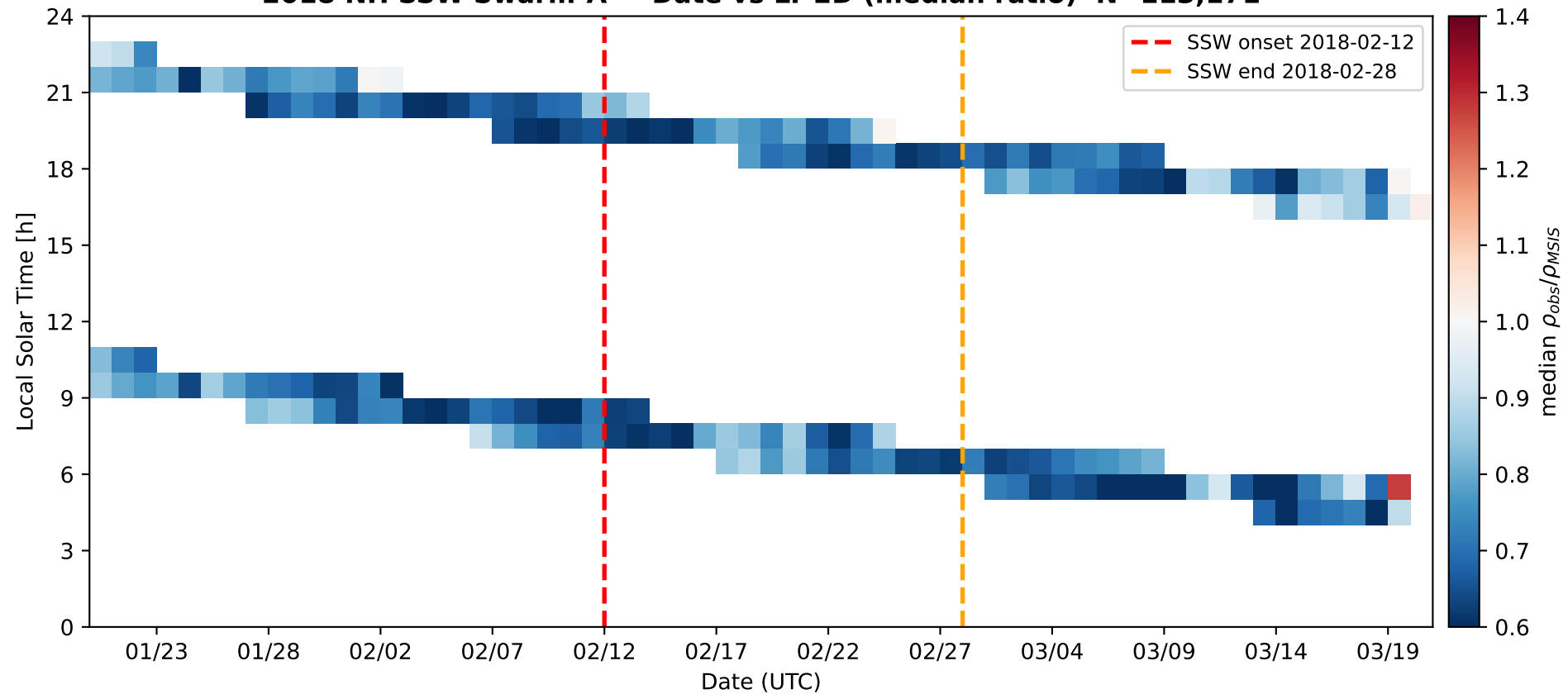
2018 NH SSW Swarm-A — Date vs LT 2D (median ratio) N=113,171
