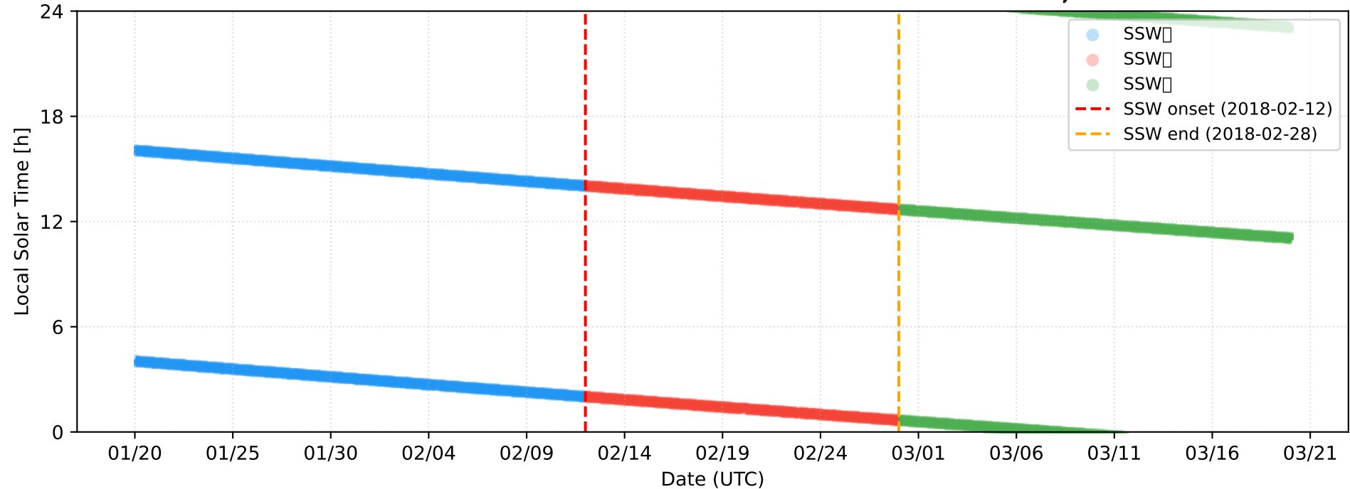
2018 NH SSW Swarm-B — Date vs Local Solar Time N=112,863
