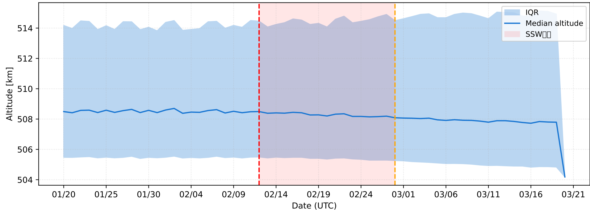
2018 NH SSW Swarm-B — Daily Altitude Distribution N=112,863
