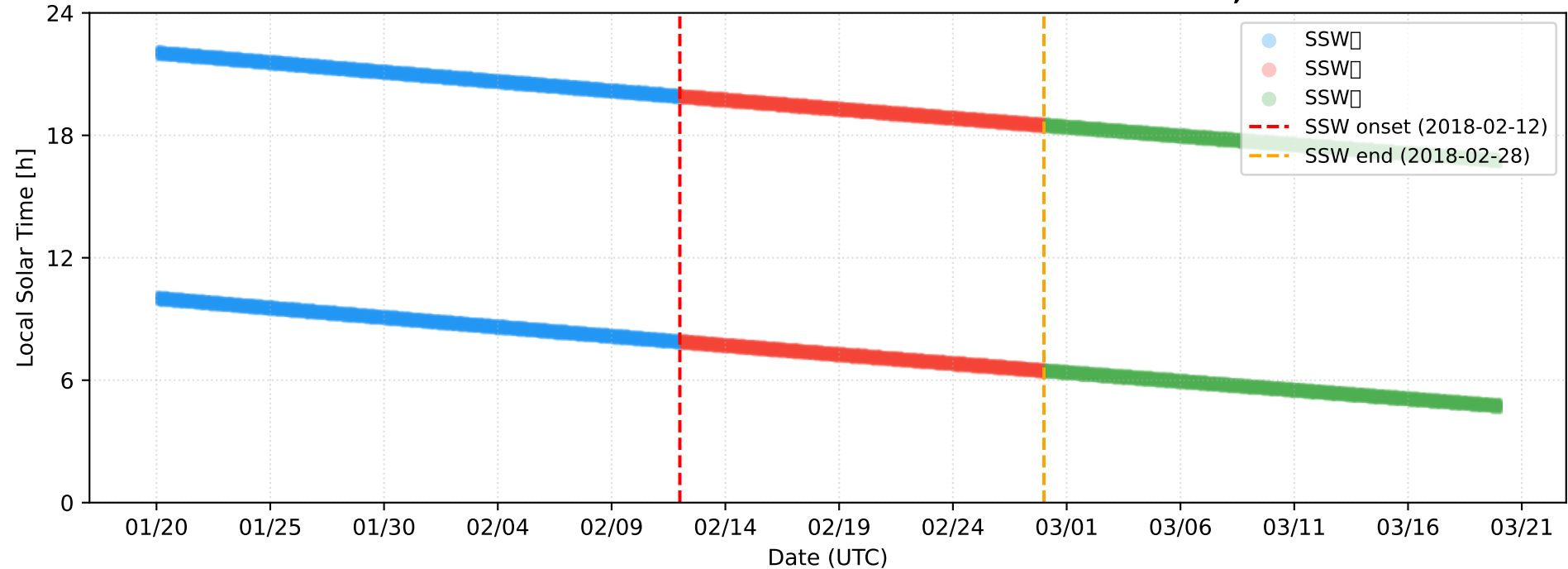
2018 NH SSW Swarm-C — Date vs Local Solar Time N=113,172
