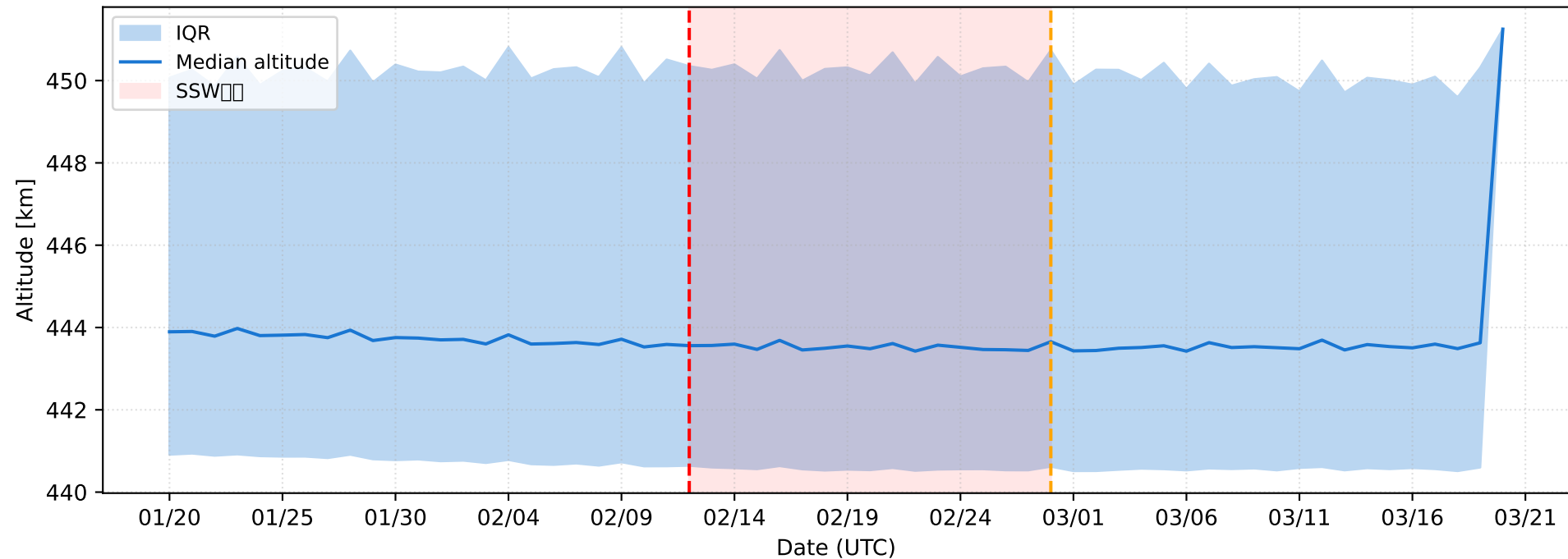
2018 NH SSW Swarm-C — Daily Altitude Distribution N=113,172
