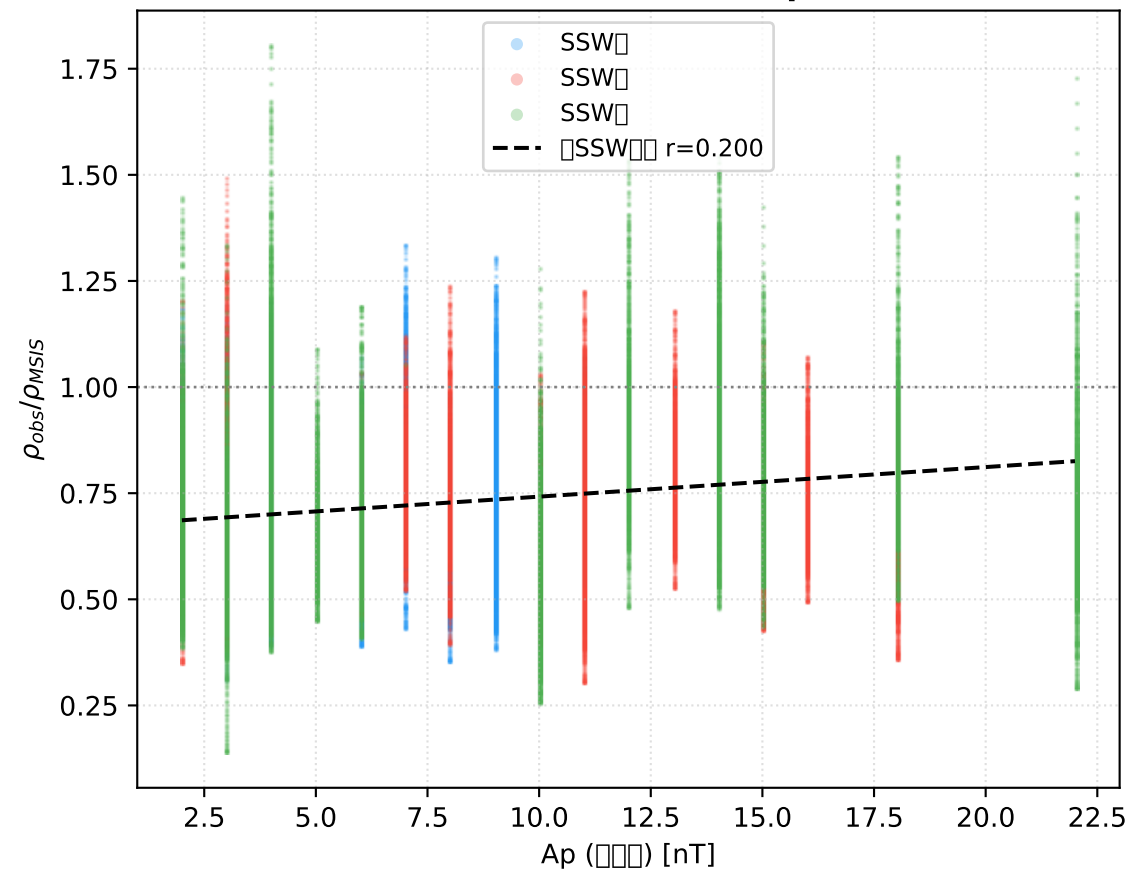
2018 NH SSW Swarm-C — Ap vs Ratio
