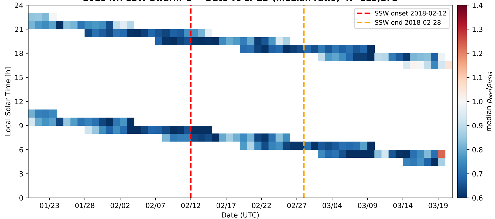
2018 NH SSW Swarm-C — Date vs LT 2D (median ratio) N=113,172
