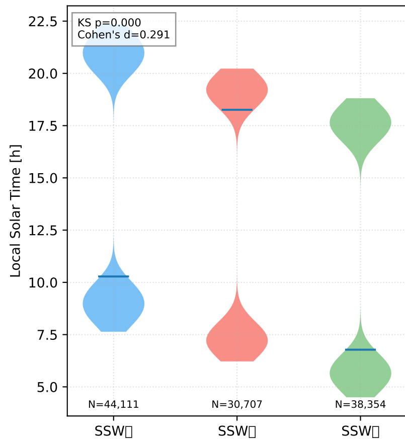
2018 NH SSW Swarm-C
