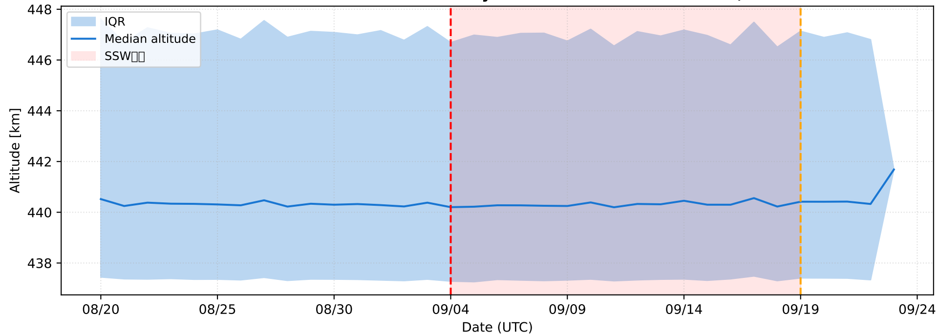
2019 SH SSW Swarm-A — Daily Altitude Distribution N=64,483
