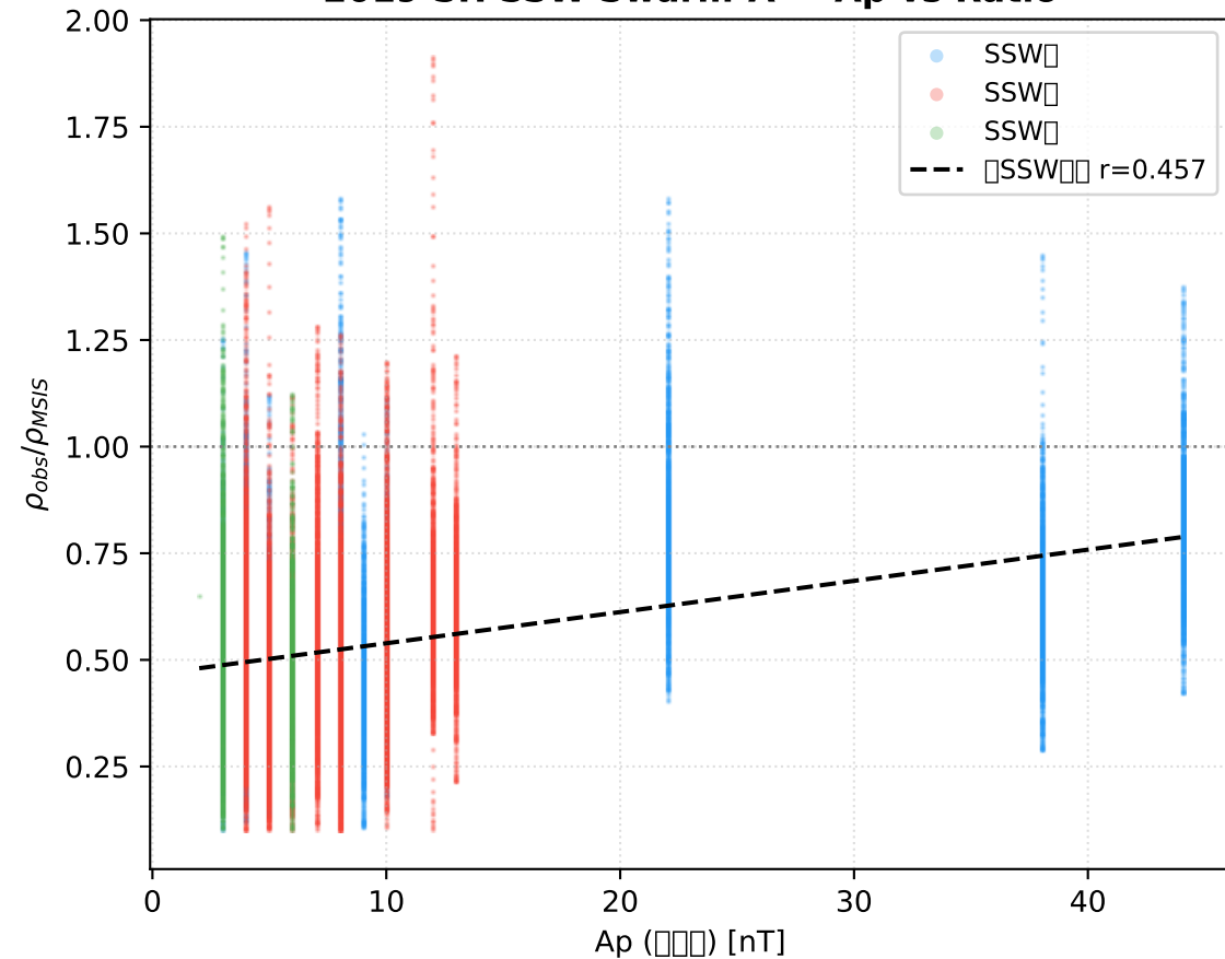
2019 SH SSW Swarm-A — Ap vs Ratio
