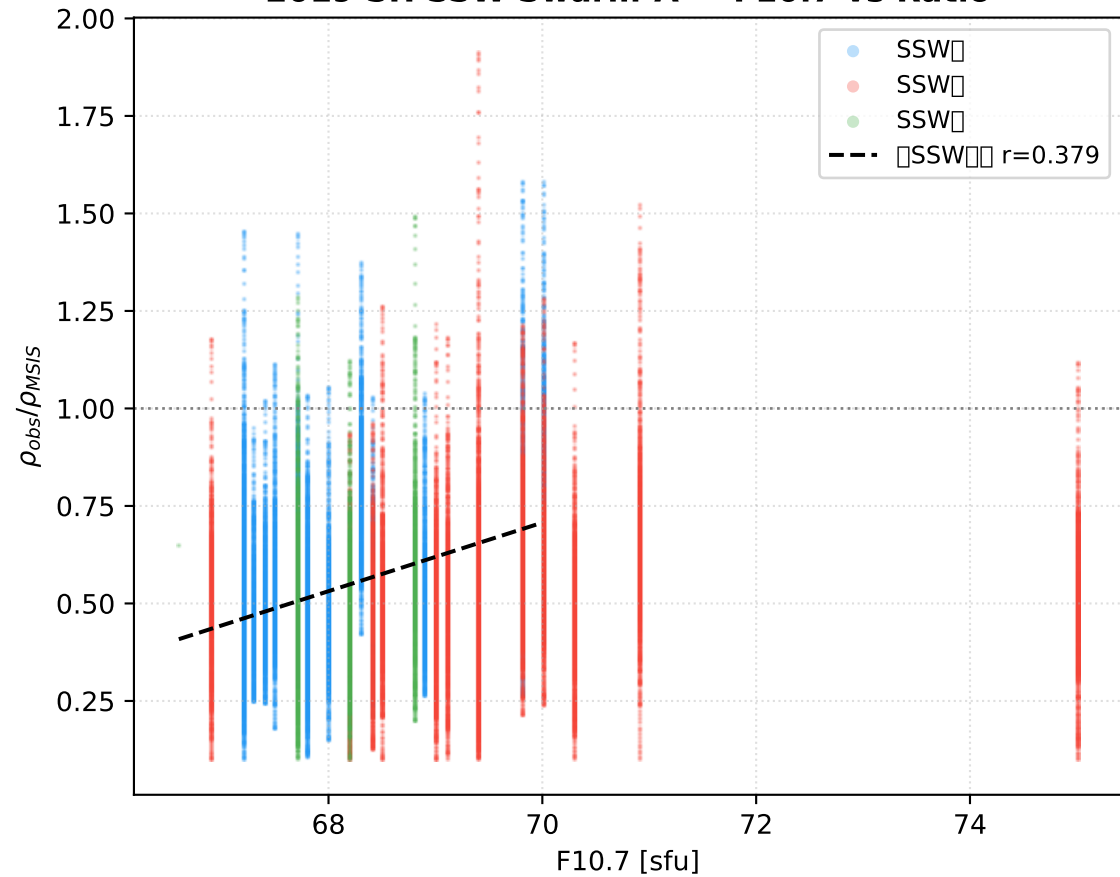
2019 SH SSW Swarm-A — F10.7 vs Ratio
