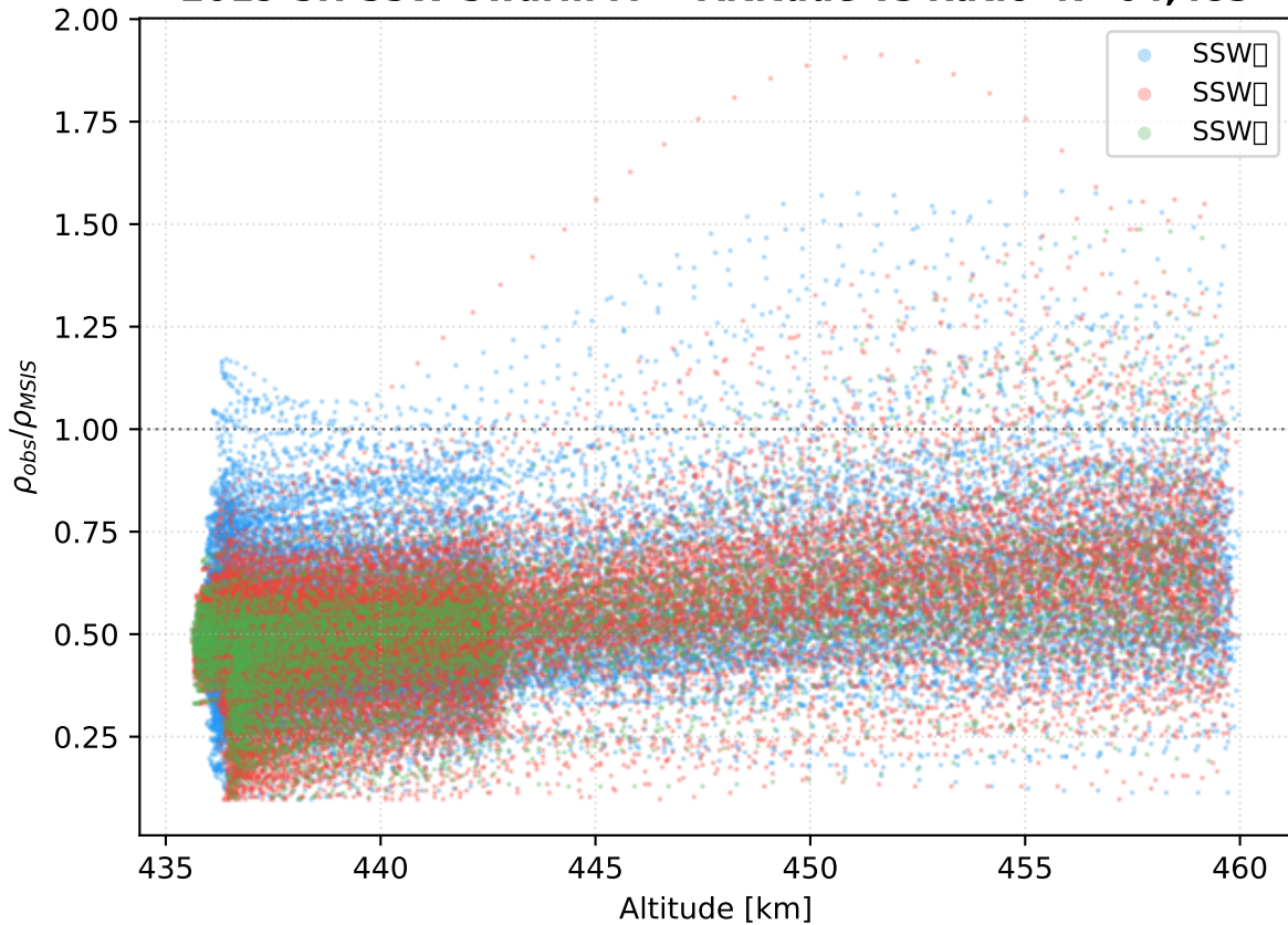
2019 SH SSW Swarm-A — Altitude vs Ratio N=64,483
