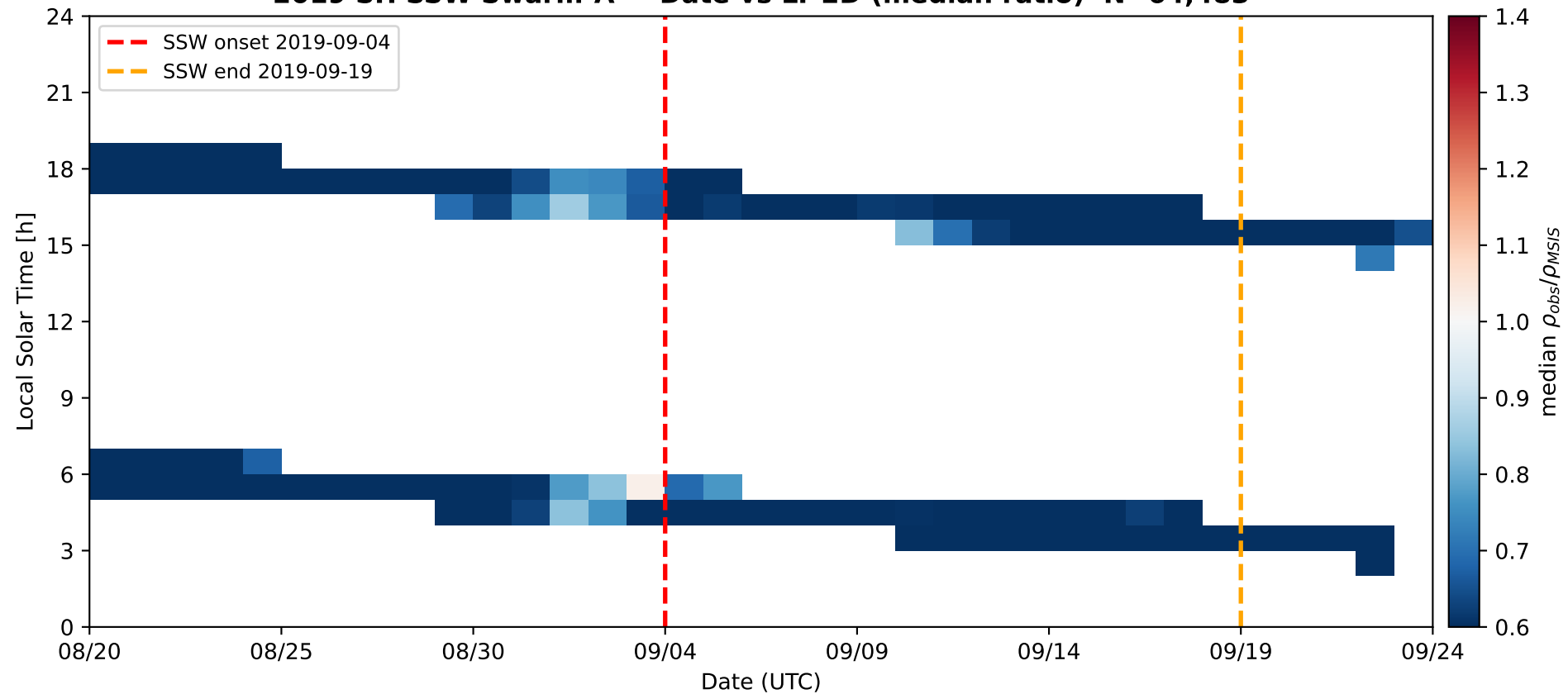
2019 SH SSW Swarm-A — Date vs LT 2D (median ratio) N=64,483
