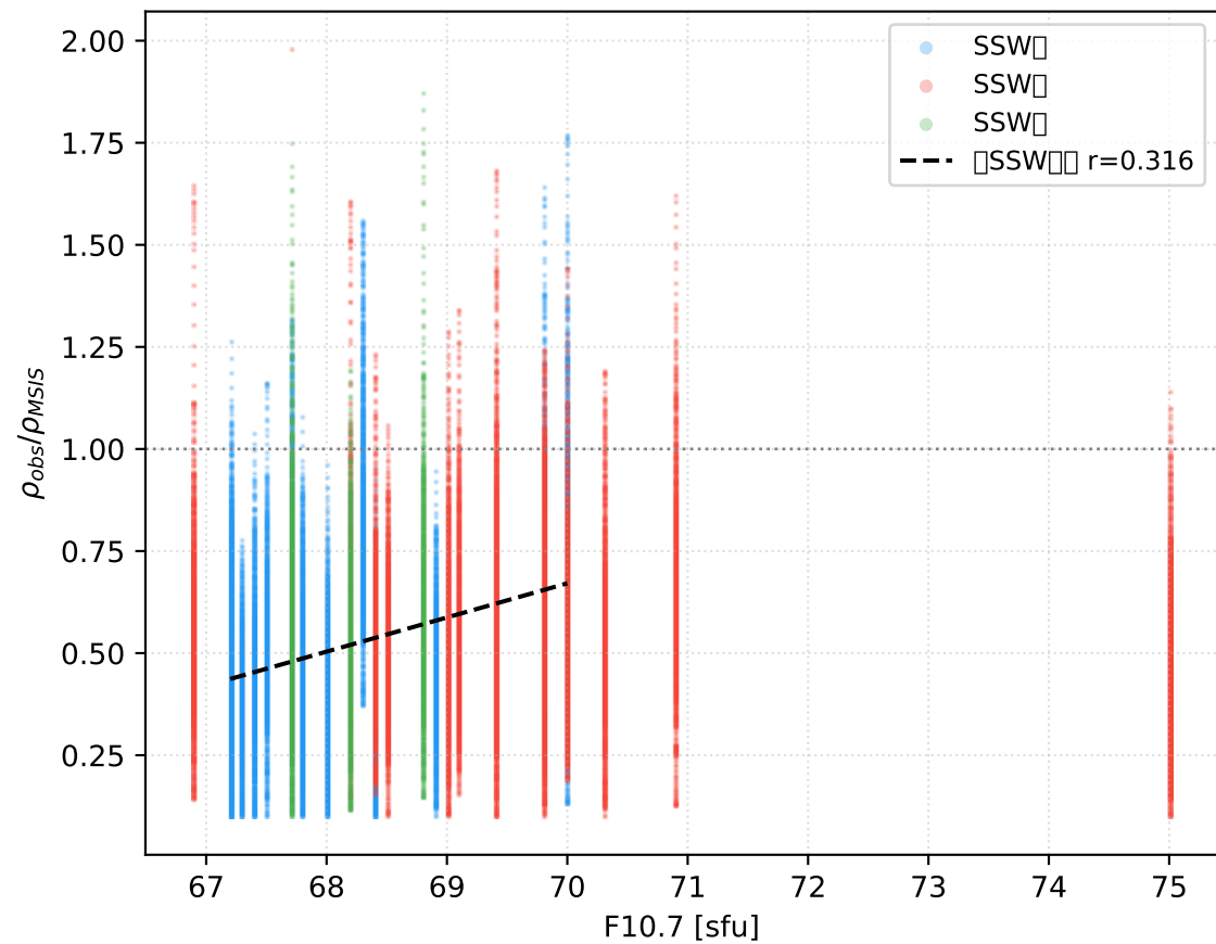
2019 SH SSW Swarm-B — F10.7 vs Ratio
