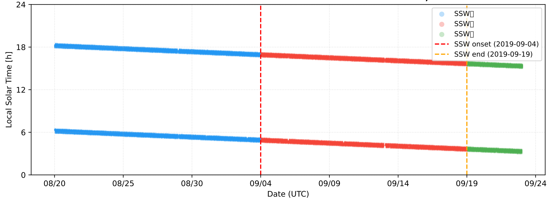
2019 SH SSW Swarm-C — Date vs Local Solar Time N=64,467
