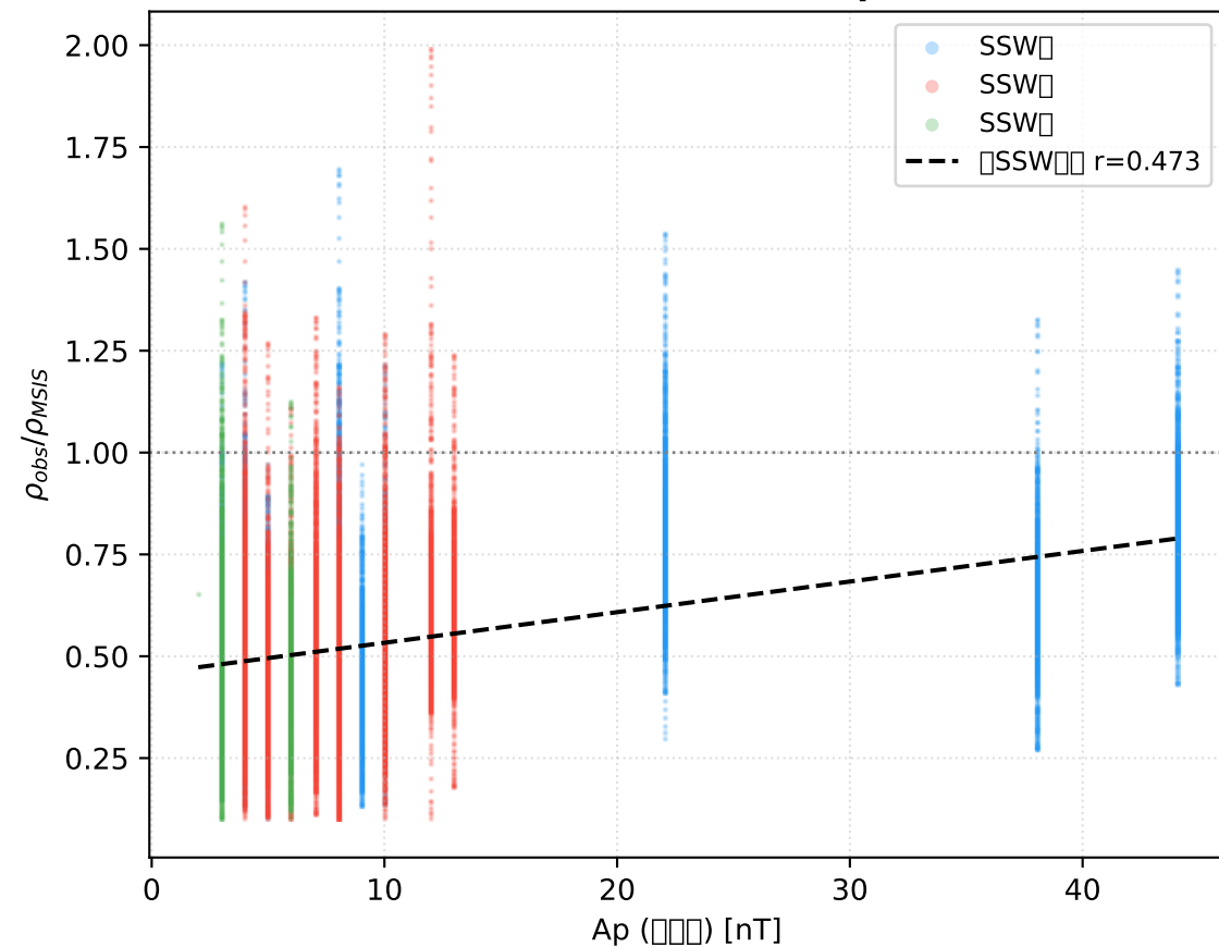
2019 SH SSW Swarm-C — Ap vs Ratio
