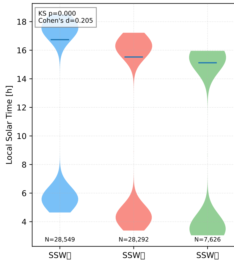
2019 SH SSW Swarm-C
