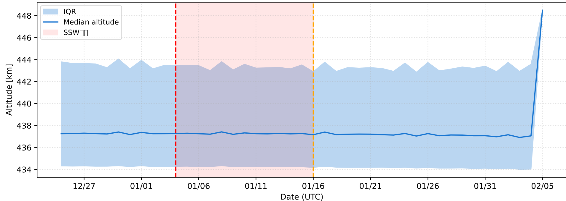
2021 NH SSW Swarm-C — Daily Altitude Distribution N=80,498
