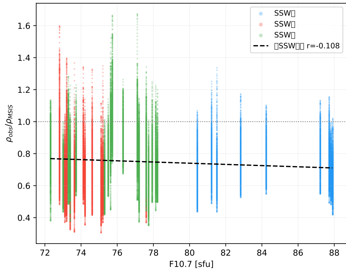
2021 NH SSW Swarm-C — F10.7 vs Ratio
