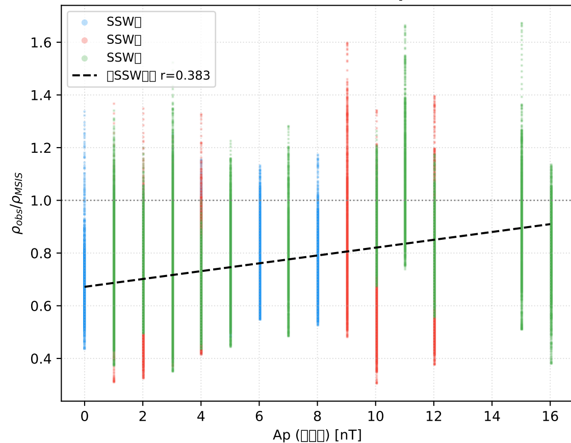
2021 NH SSW Swarm-C — Ap vs Ratio
