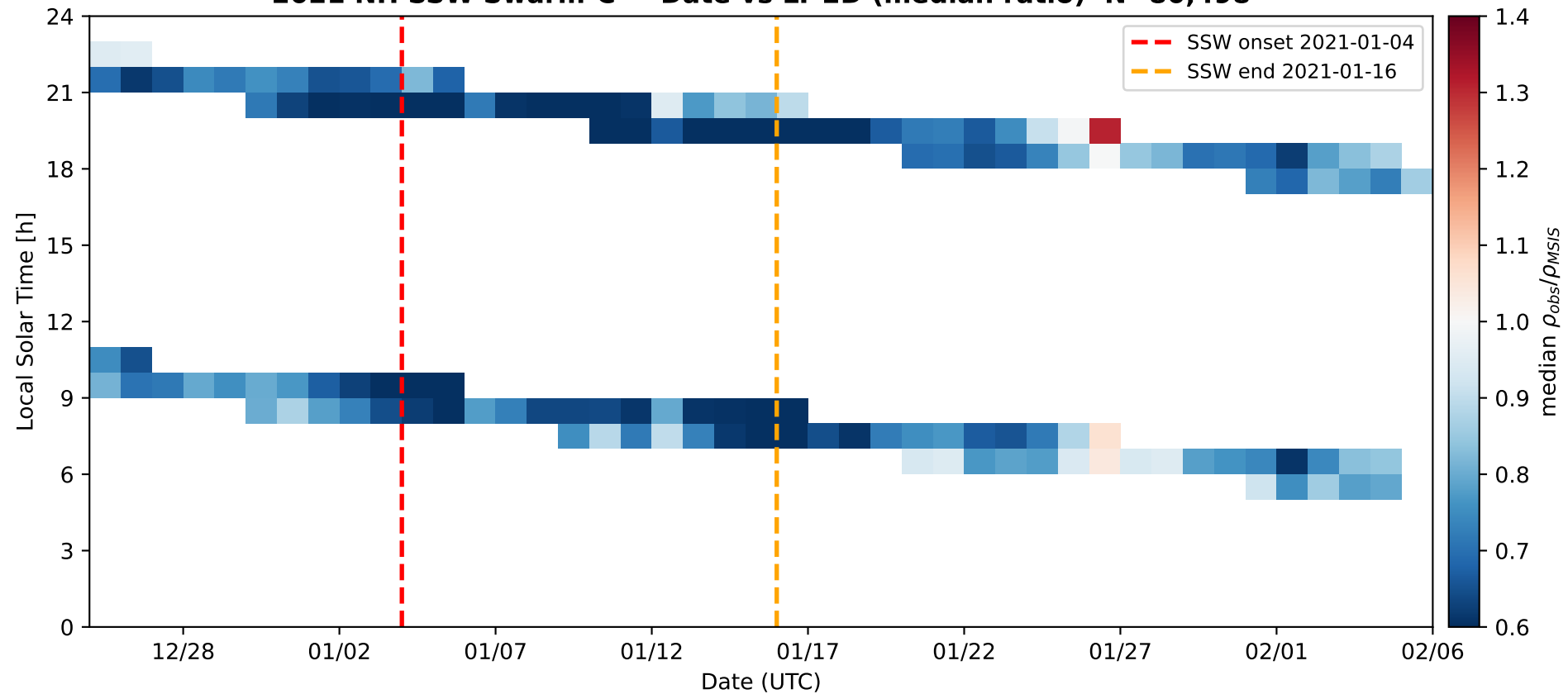
2021 NH SSW Swarm-C — Date vs LT 2D (median ratio) N=80,498
