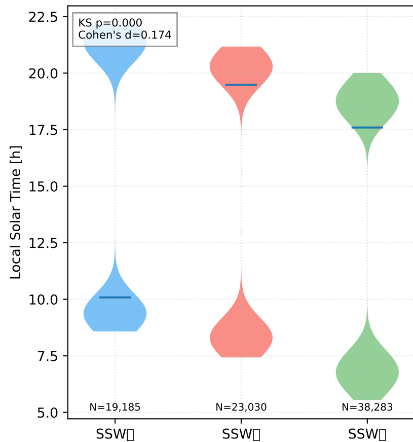
2021 NH SSW Swarm-C
