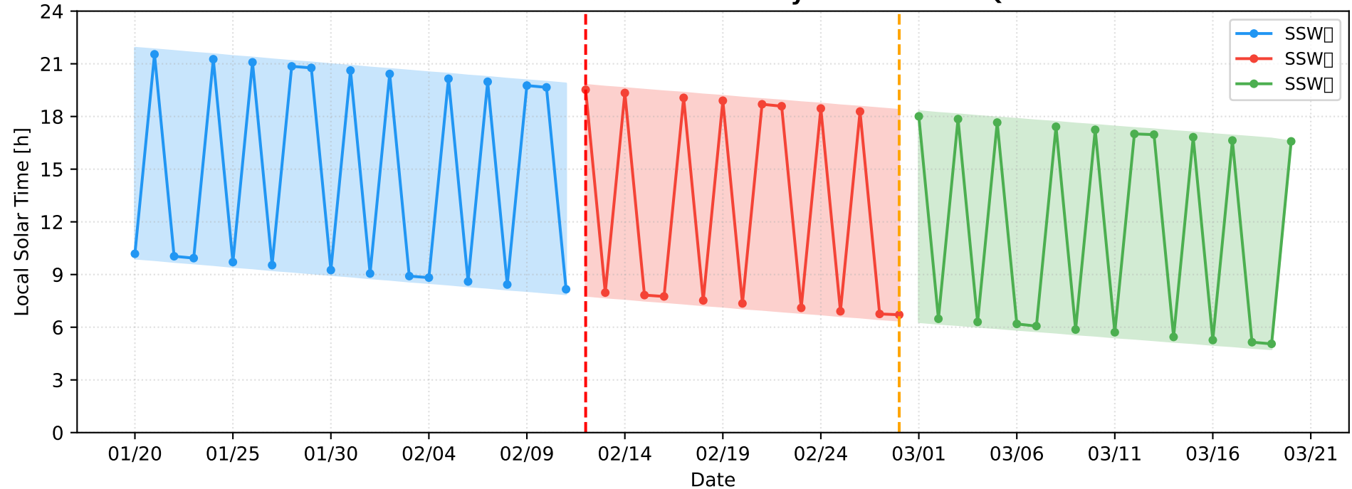
2018 NH SSW Swarm-A — Daily Median LT \pm IQR
