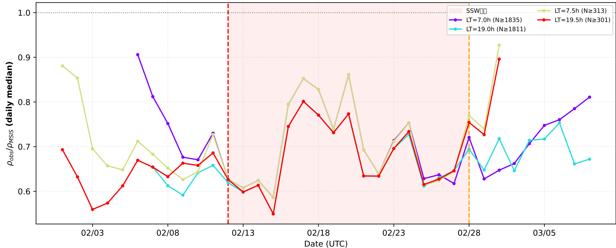
2018 NH SSW Swarm-A — Multi-LT Overlay \pm 1.0h bins
