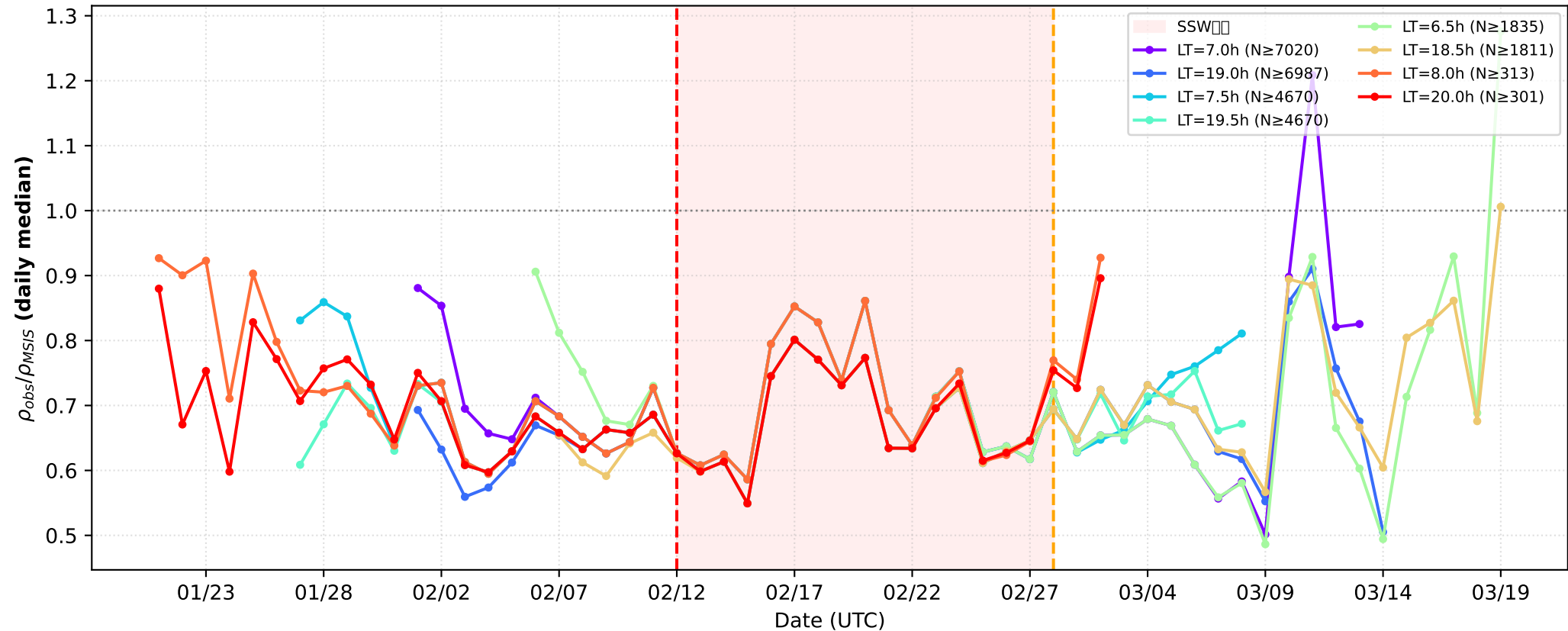
2018 NH SSW Swarm-A — Multi-LT Overlay \pm 1.5h bins
