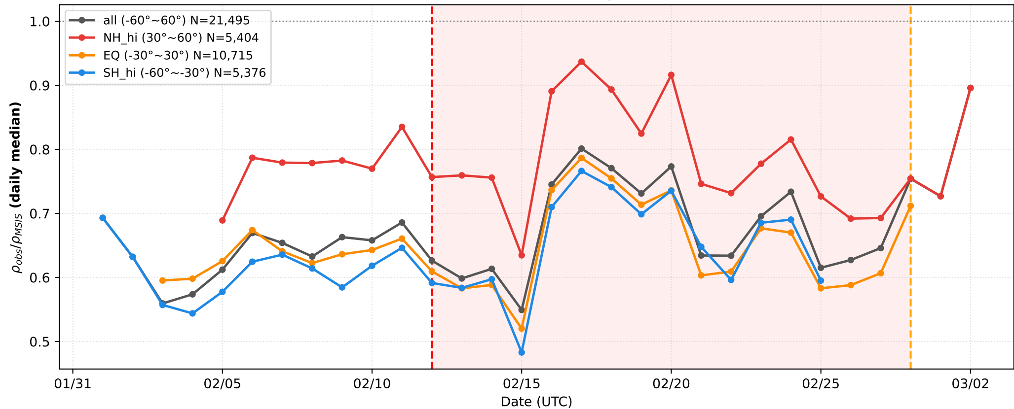
2018 NH SSW Swarm-A — Lat-band Comparison LT=19.5h \pm 1.0h
