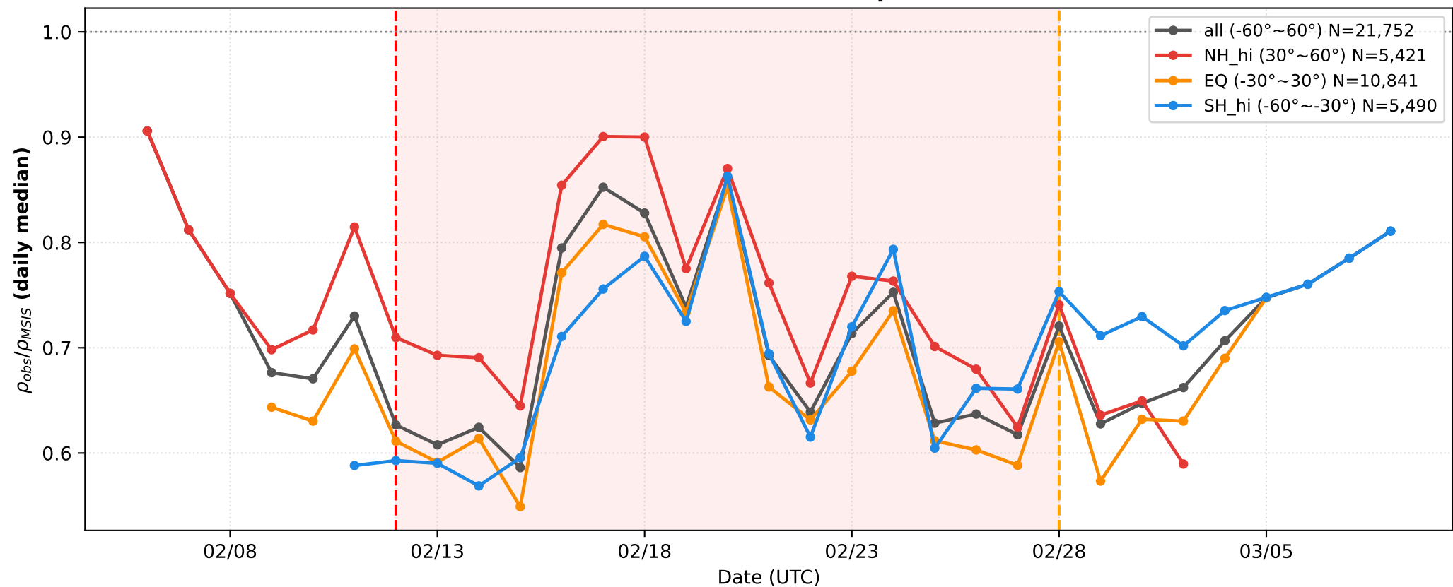
2018 NH SSW Swarm-A — Lat-band Comparison LT=7.0h ±1.0h
