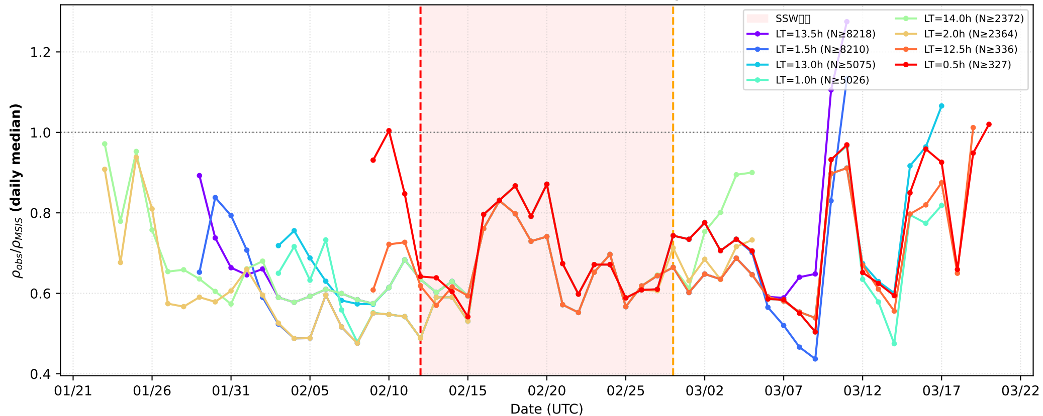
2018 NH SSW Swarm-B — Multi-LT Overlay \pm 1.5h bins
