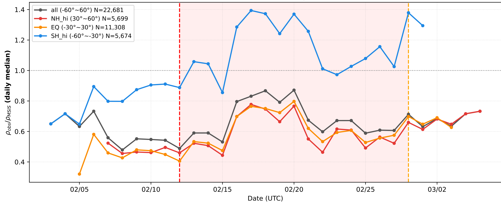
2018 NH SSW Swarm-B — Lat-band Comparison LT=1.5h ±1.0h
