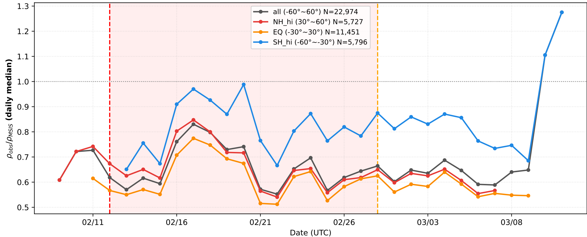
2018 NH SSW Swarm-B — Lat-band Comparison LT=13.0h \pm 1.0h
