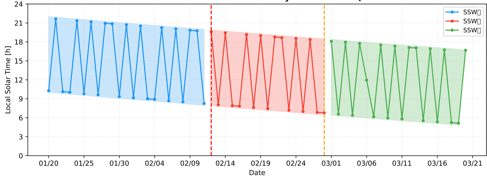
2018 NH SSW Swarm-C — Daily Median LT \pm IQR
