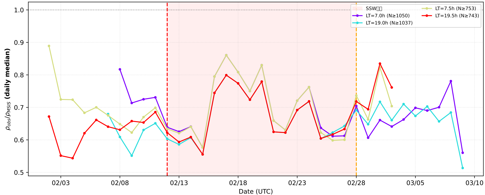
2018 NH SSW Swarm-C — Multi-LT Overlay \pm 1.0h bins
