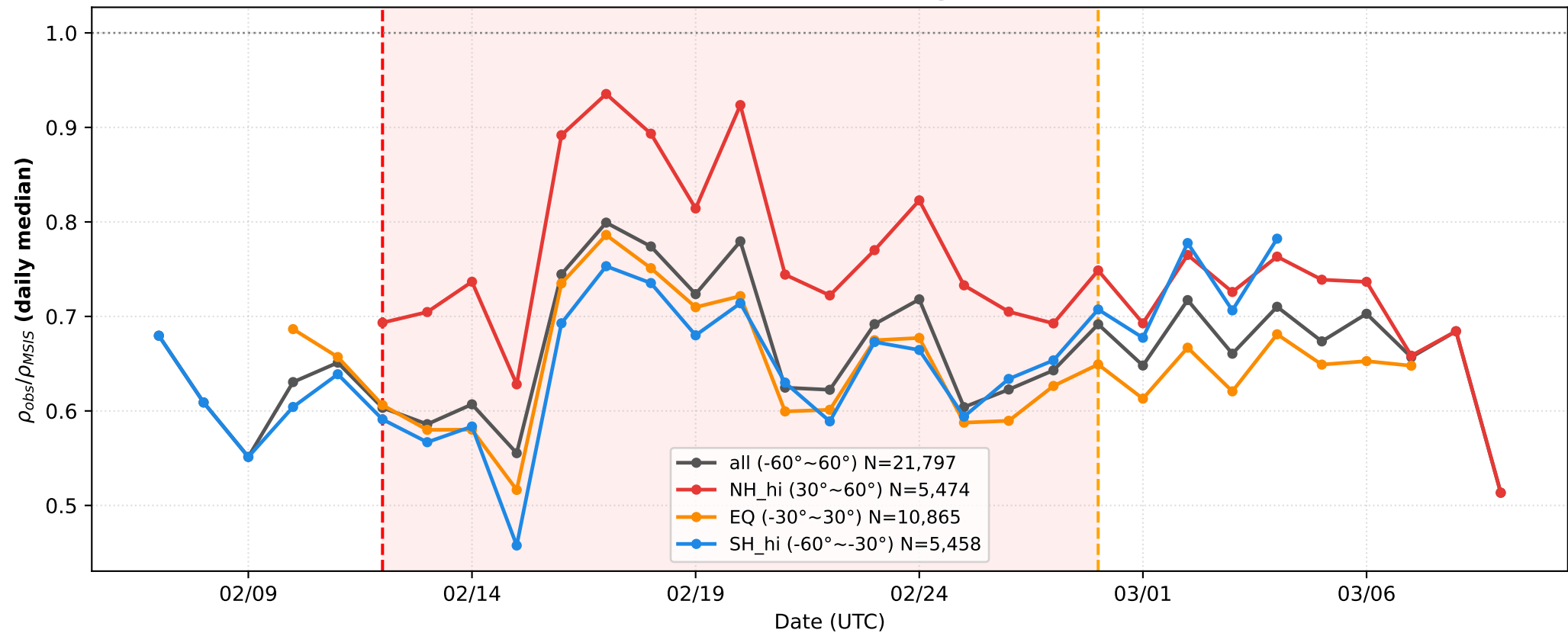
2018 NH SSW Swarm-C — Lat-band Comparison LT=19.0h \pm 1.0h
