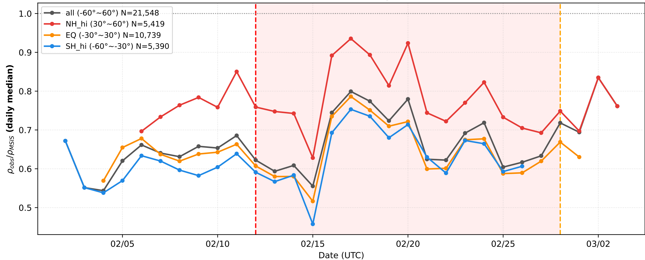
2018 NH SSW Swarm-C — Lat-band Comparison LT=19.5h ±1.0h
