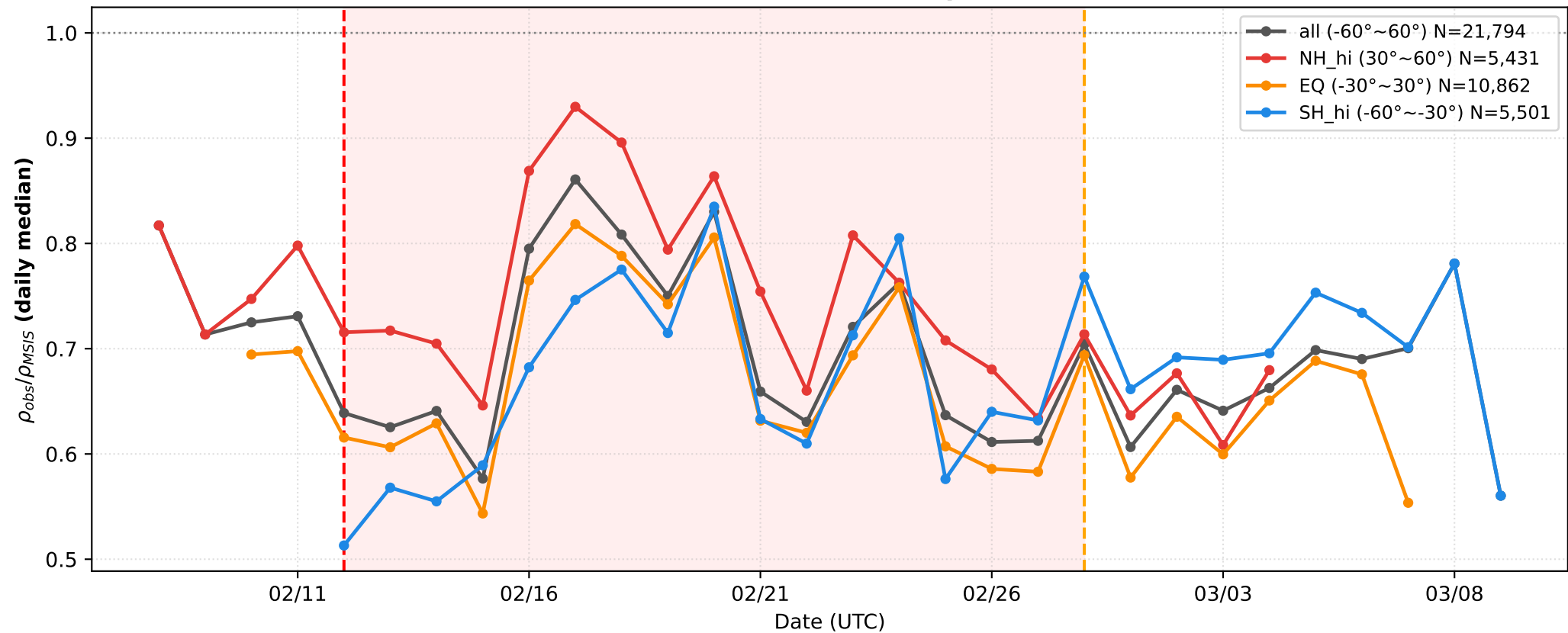
2018 NH SSW Swarm-C — Lat-band Comparison LT=7.0h ±1.0h
