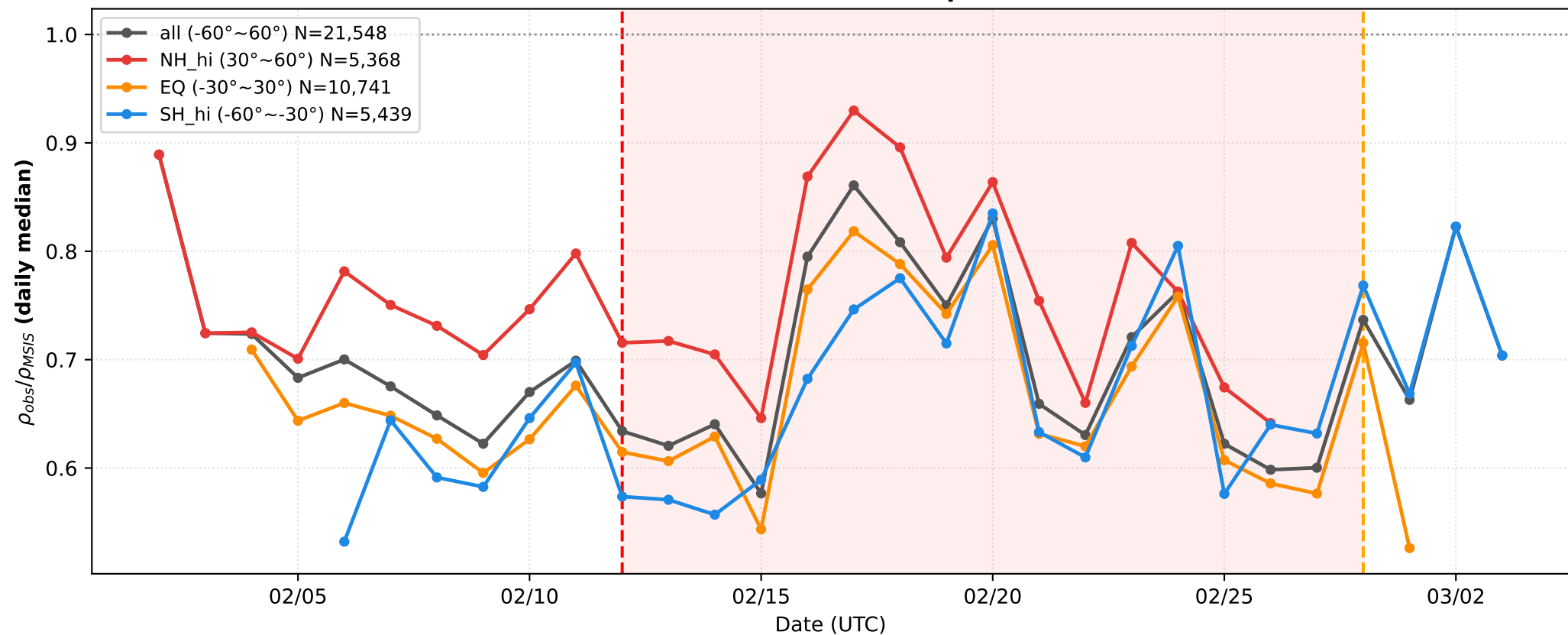
2018 NH SSW Swarm-C — Lat-band Comparison LT=7.5h \pm 1.0h
