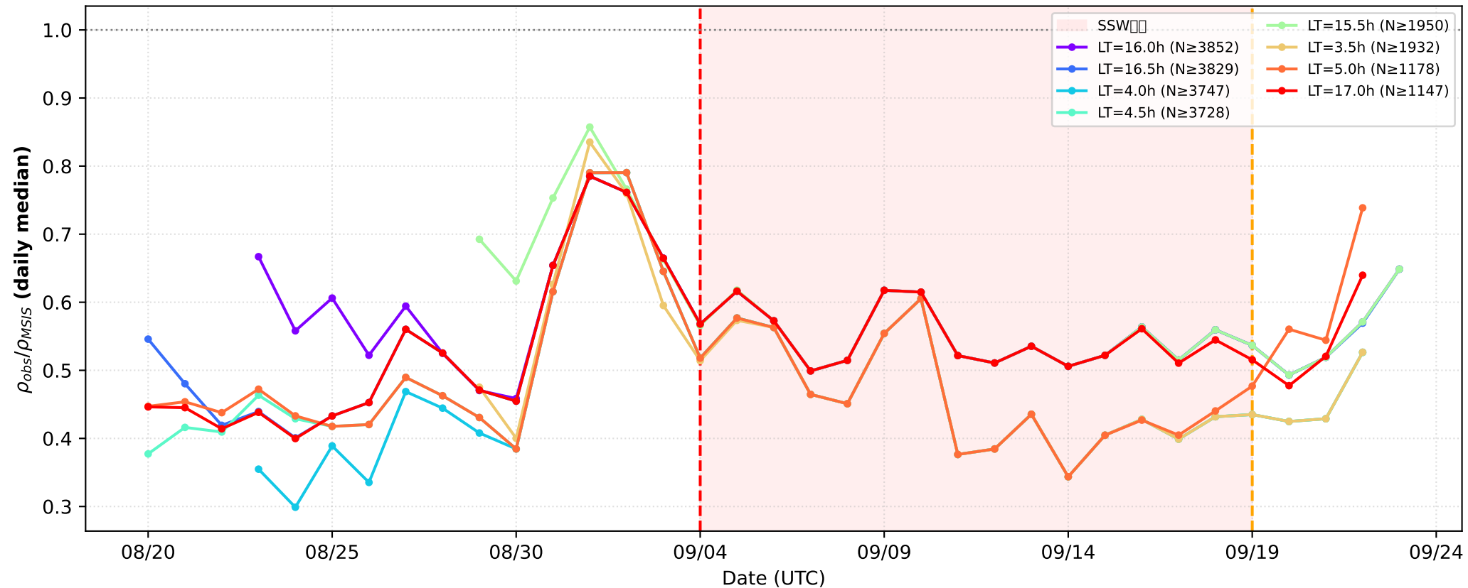
2019 SH SSW Swarm-A — Multi-LT Overlay \pm 1.5h bins
