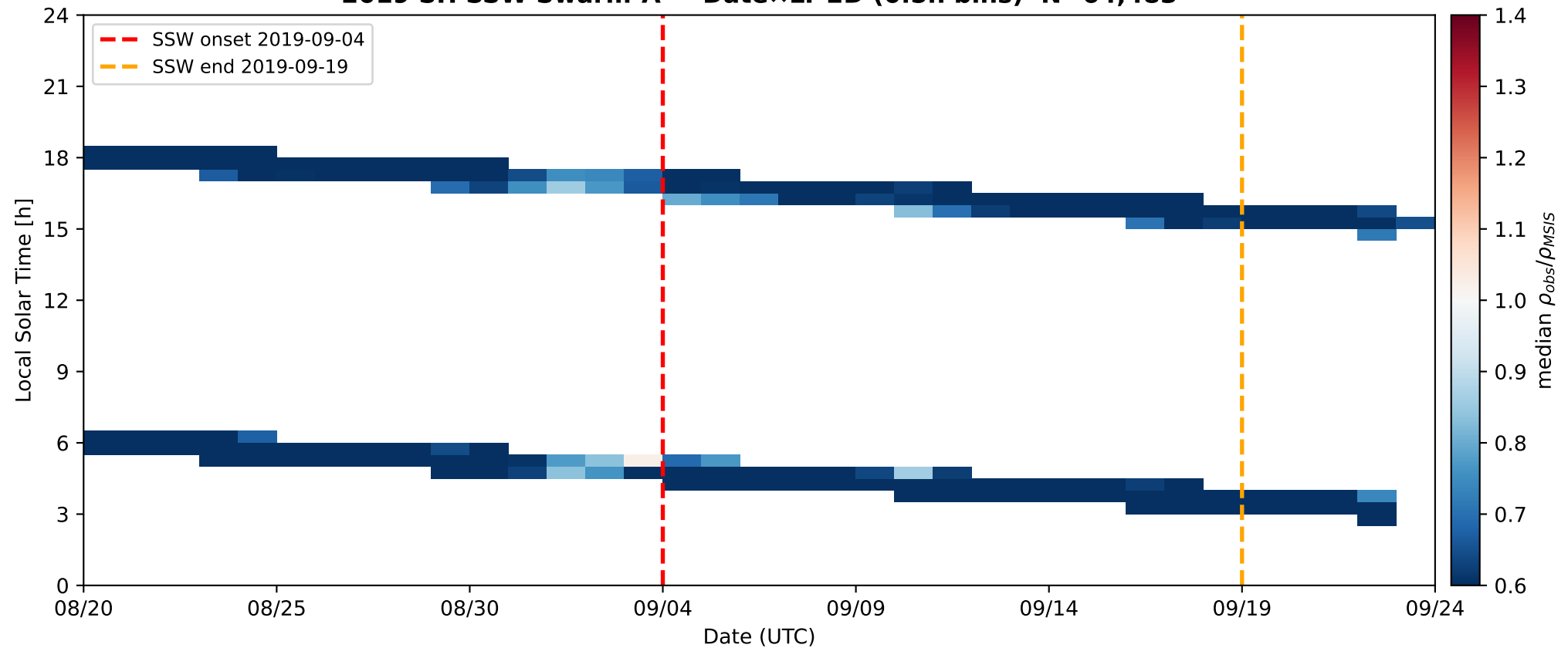
2019 SH SSW Swarm-A — Date×LT 2D (0.5h bins) N=64,483
