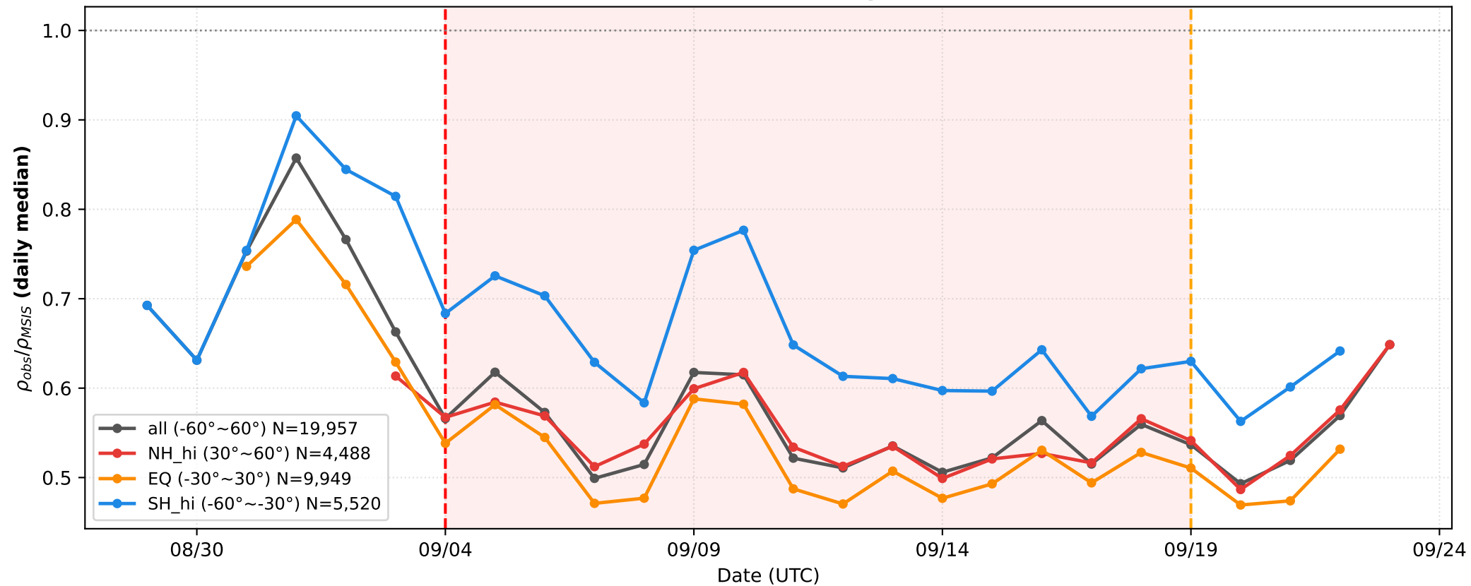
2019 SH SSW Swarm-A — Lat-band Comparison LT=16.0h \pm 1.0 h
