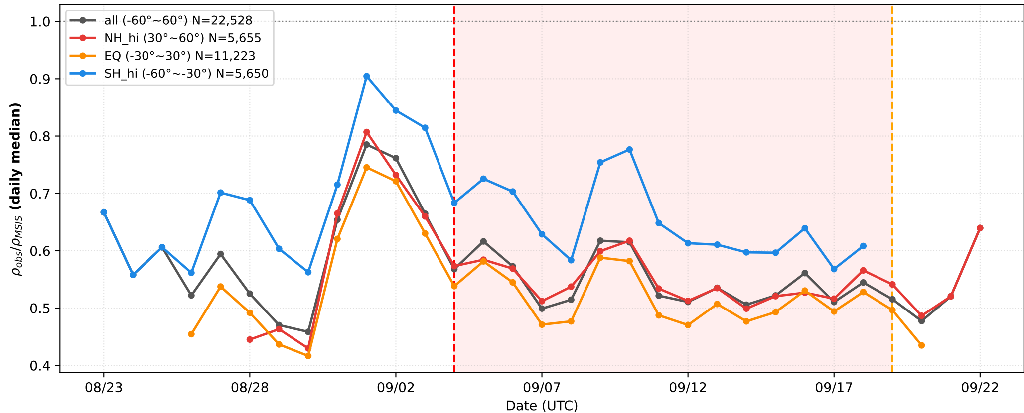
2019 SH SSW Swarm-A — Lat-band Comparison LT=16.5h \pm 1.0h
