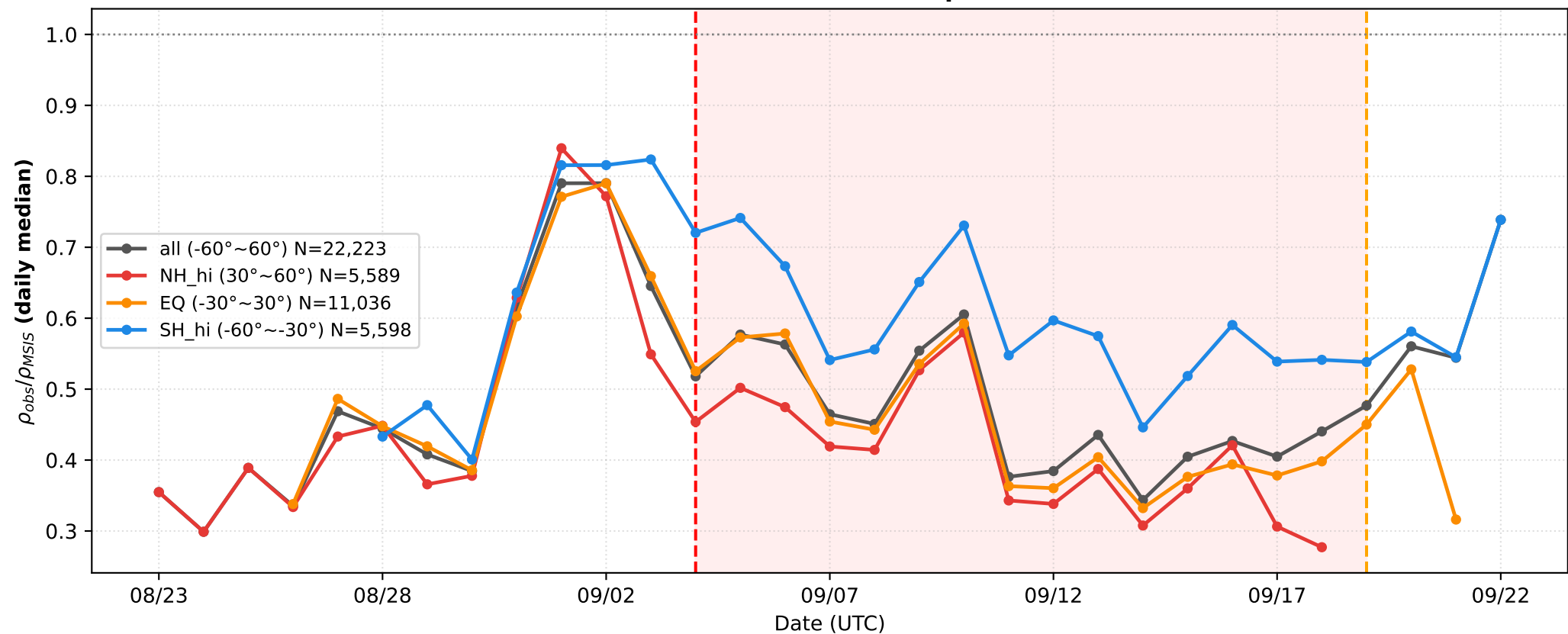
2019 SH SSW Swarm-A — Lat-band Comparison LT=4.5h \pm 1.0h
