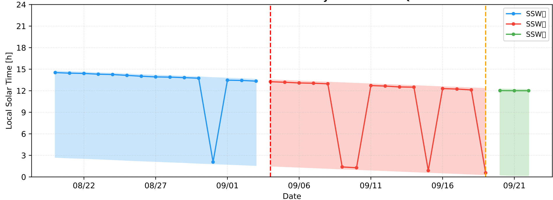
2019 SH SSW Swarm-B — Daily Median LT \pm IQR
