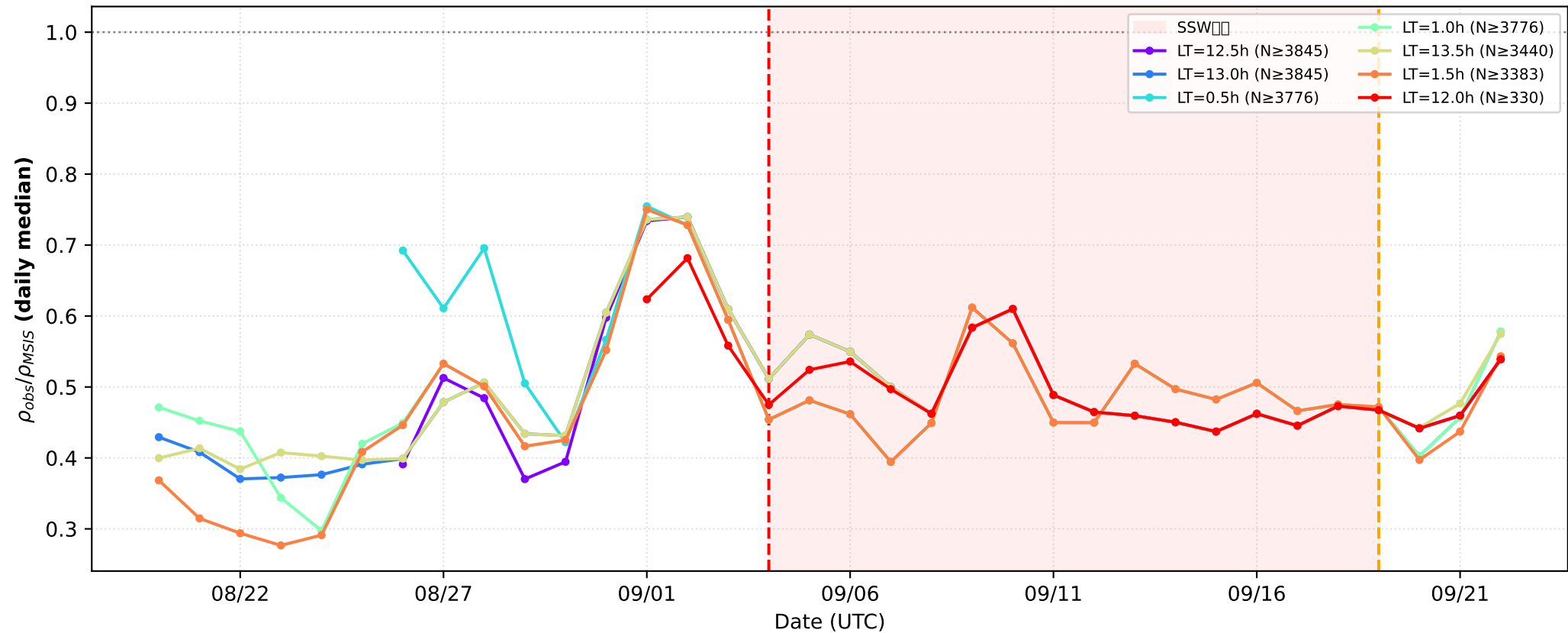
2019 SH SSW Swarm-B — Multi-LT Overlay \pm 1.5h bins
